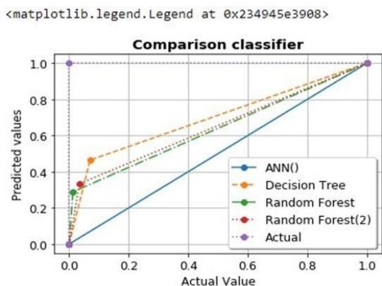
Figure 5: Comparing the predicted and actual values from a classifier across various algorithms
