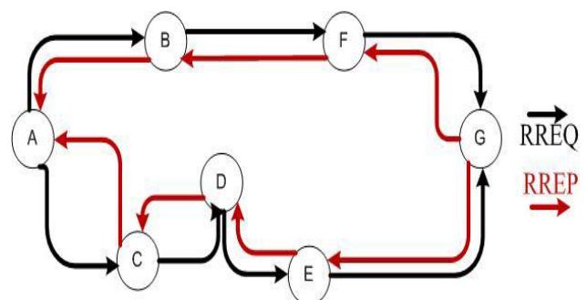
Figure 2.3 AODV Route
