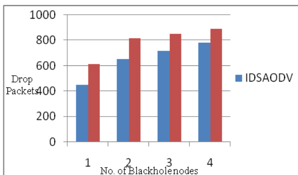
Figure 4(a) Drop Packets
