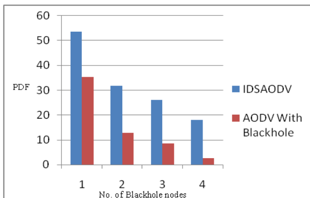
Fig. 4(b) Packet Delivery Ratio
