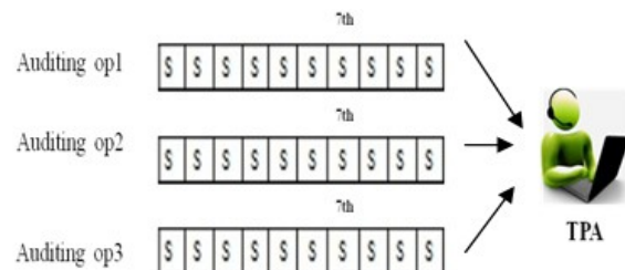
Figure 2: TPA audits the integrity of shared data using with oruta. A and B share a file in the cloud
