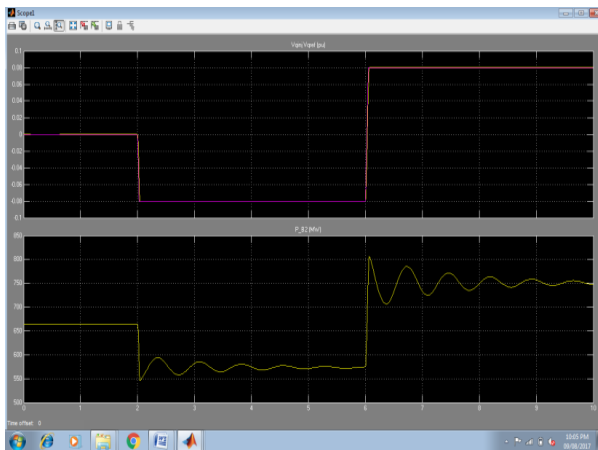
Figure 4: Shows the facility obtained in the least the buses B1, B2, B3 and B4 while not SSSC.
