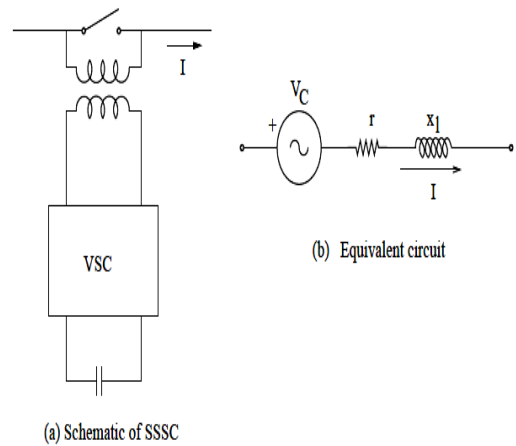
Figure 1. Schematic of SSSC. [2]
