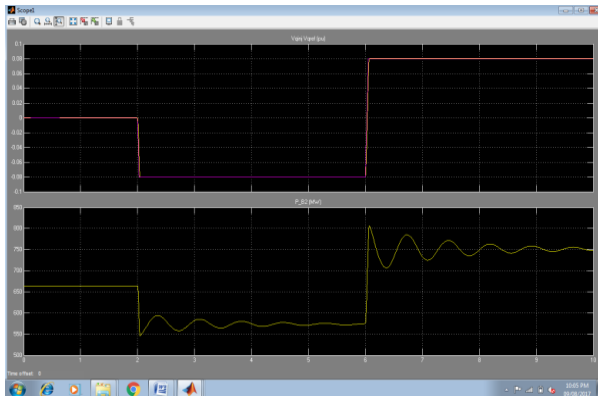
Figure 3 Illustrates, the Facility Obtained at Bus B2 while not SSSC.
