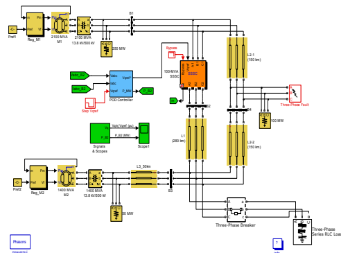
Figure 2: Simulink Diagram Representation of Proposed Work.
