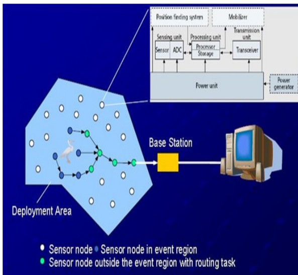
Figure 1: WSNs components overview [7]
