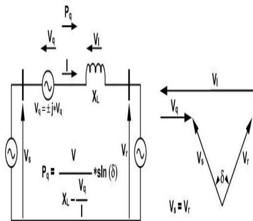
Figure 4: Simplified Diagram of Series Compensation with the Phasor Diagram. [11]
