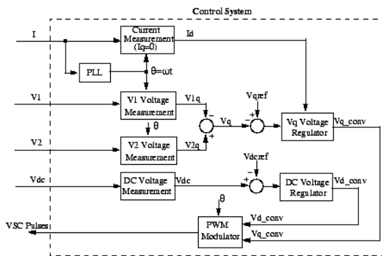
Figure 2: System Diagram of a SSSC.
