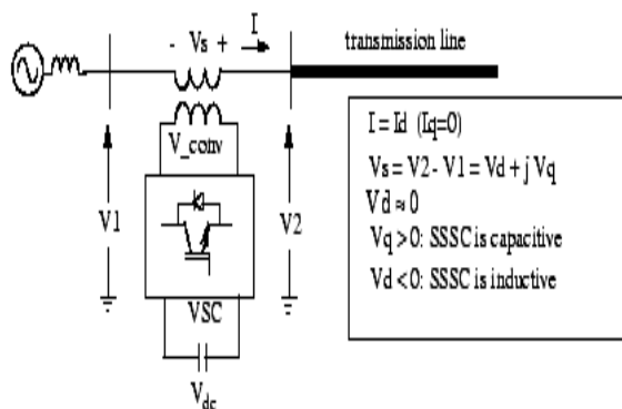
Figure 1: Single-line Diagram of a SSSC.
