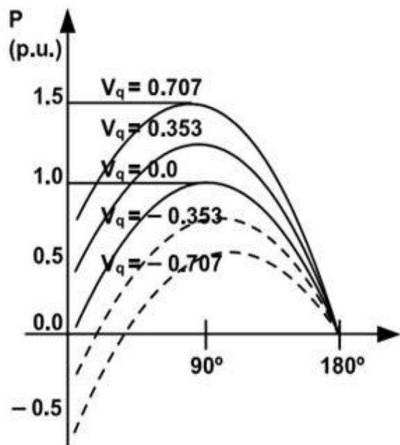
Figure 5: Transmitted power versus transmitted angle as a function of series compensation [12]
