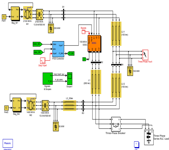
Figure 6: Simulink Diagram Representation of Proposed Work.
