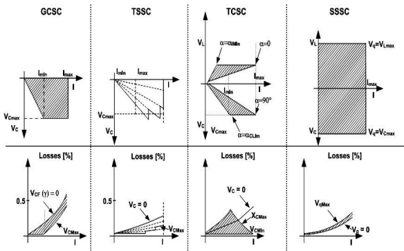
Figure 3: Comparisons of Variable Type Series Compensators to Converter Type Series Compensator [8]
