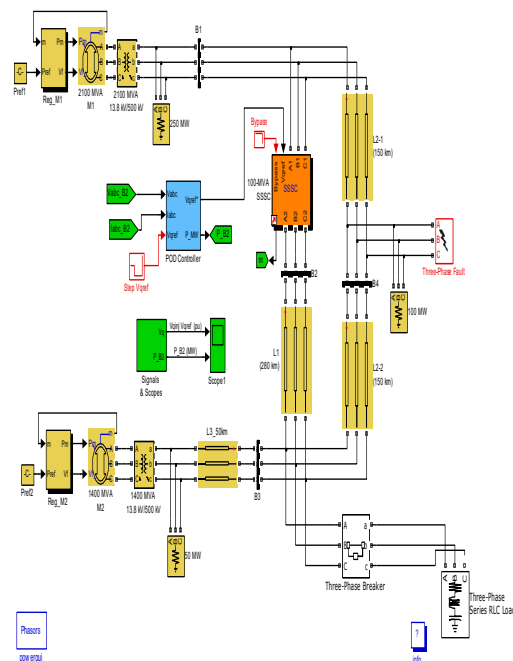
Figure 2: Simulink diagram representation of proposed work.
