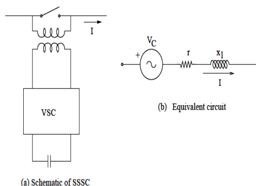
Figure 1. Schematic of SSSC. [2]
