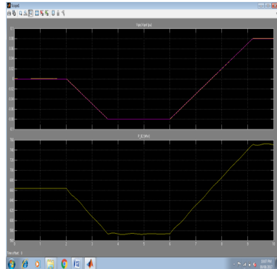
Figure 5: illustrates, the facility obtained at bus B2 while not SSSC.
